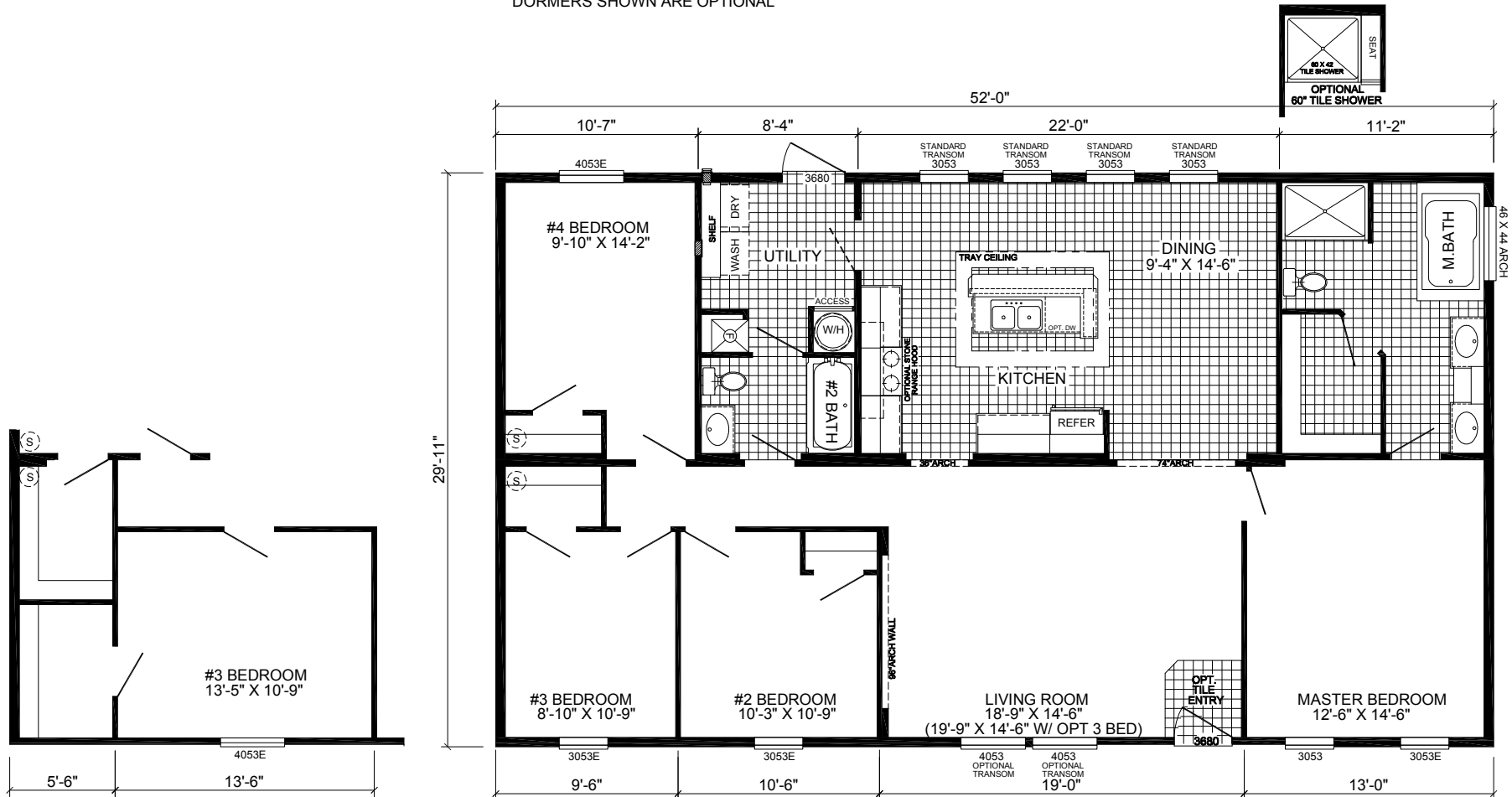
P-3524E 4-BEDROOM / 2-BATH 32 x 56 - Approx. 1549 Sq. Ft.
